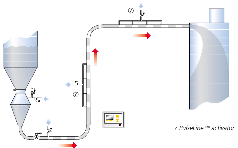
Chemical products: Pneumatic dense phase conveying with weighing and throughput recording.
